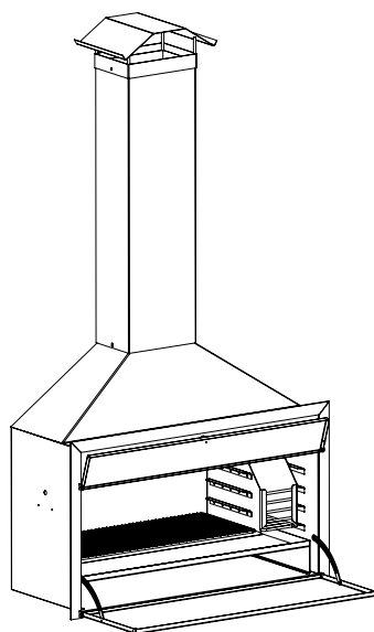
FRONT VIEW OF I200 BUILT IN BRAAI
