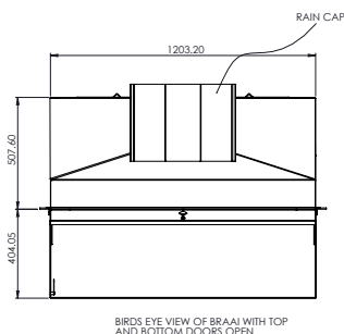
BIRD'S EYE VIEW OF BRAAI WITH TOP AND BOTTOM DOORS OPEN
